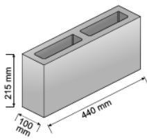
4" Hollow
