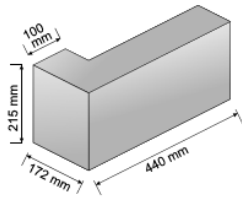
L Block
