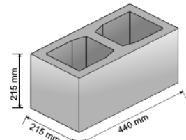
9" Cavity
