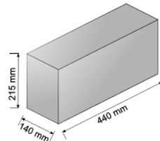
6" Solid
