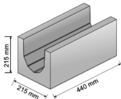
U Block
