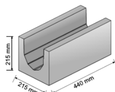
U Block
