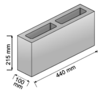
4" Hollow
