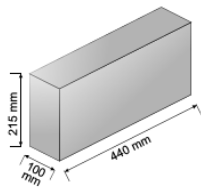
4" Solid
