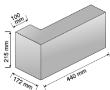
L Block
