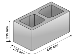
9" Cavity
